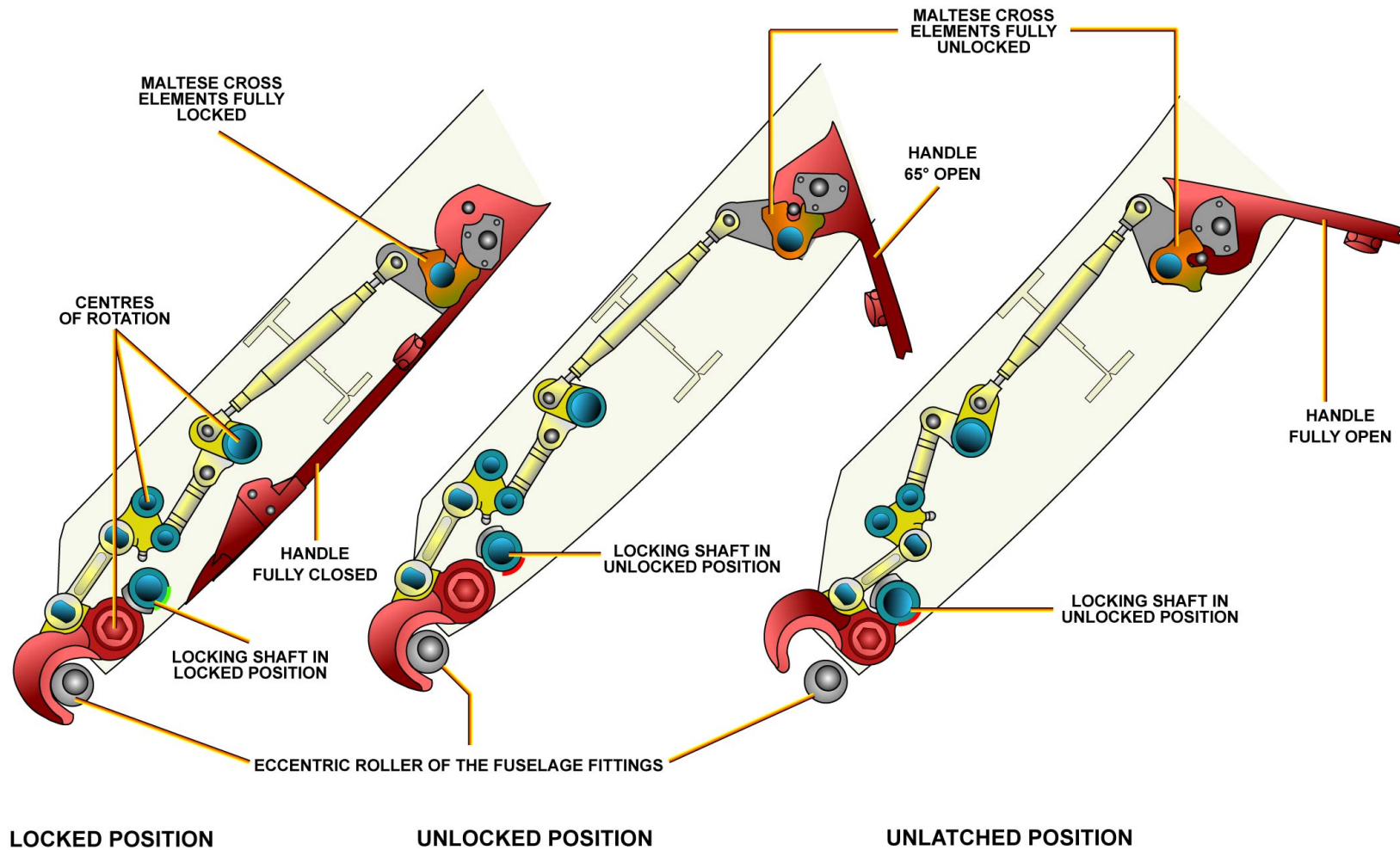
UNLOCKING AND UNLATCHING OPERATION - LOCKED POSITION ... UNLATCHED POSITION
