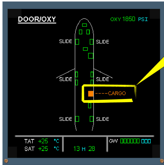
DOOR ECAM PAGE
