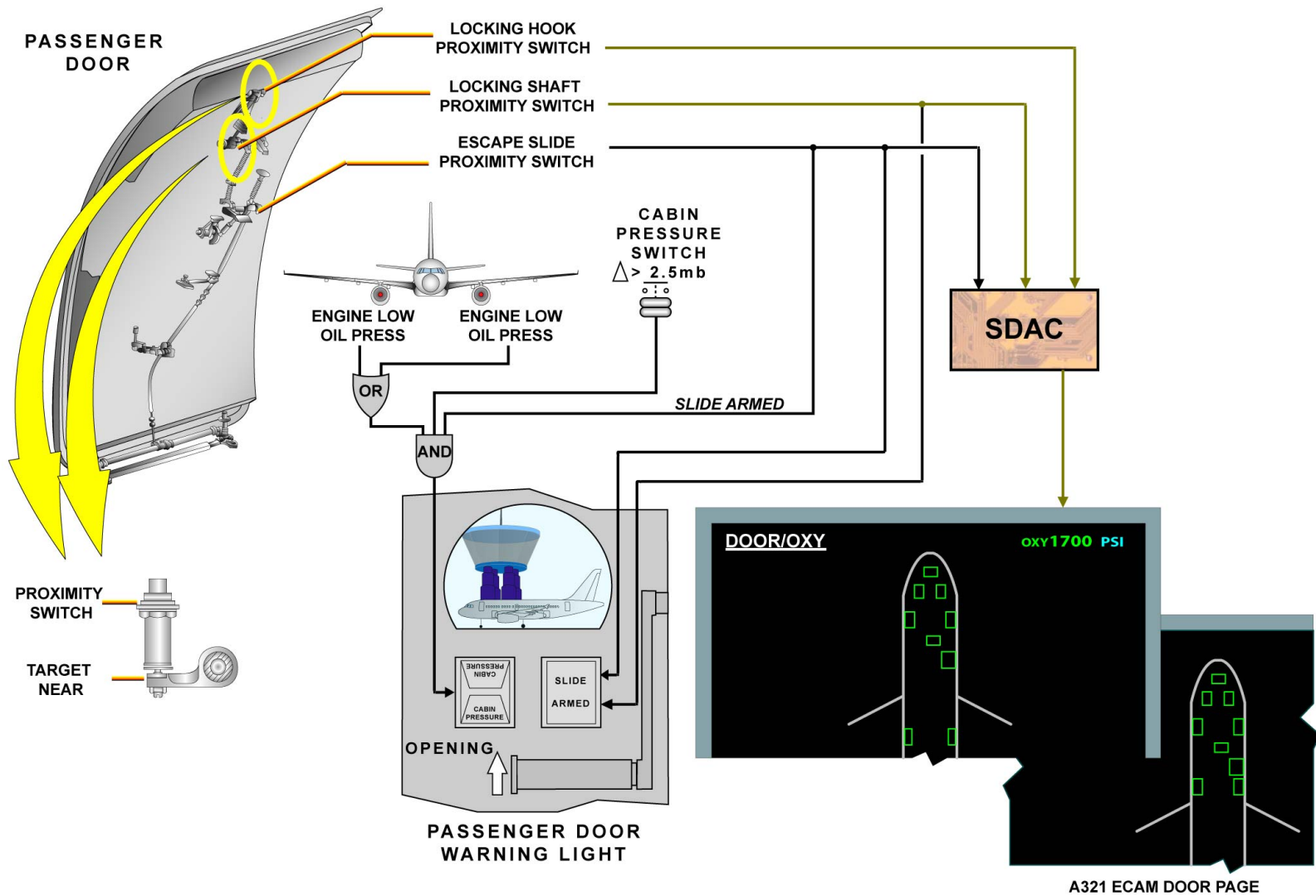
PASSENGER DOORS - DOOR INDICATING AND WARNING - PRINCIPLE &amp; DOOR INDICATING AND WARNING - LOCKED
