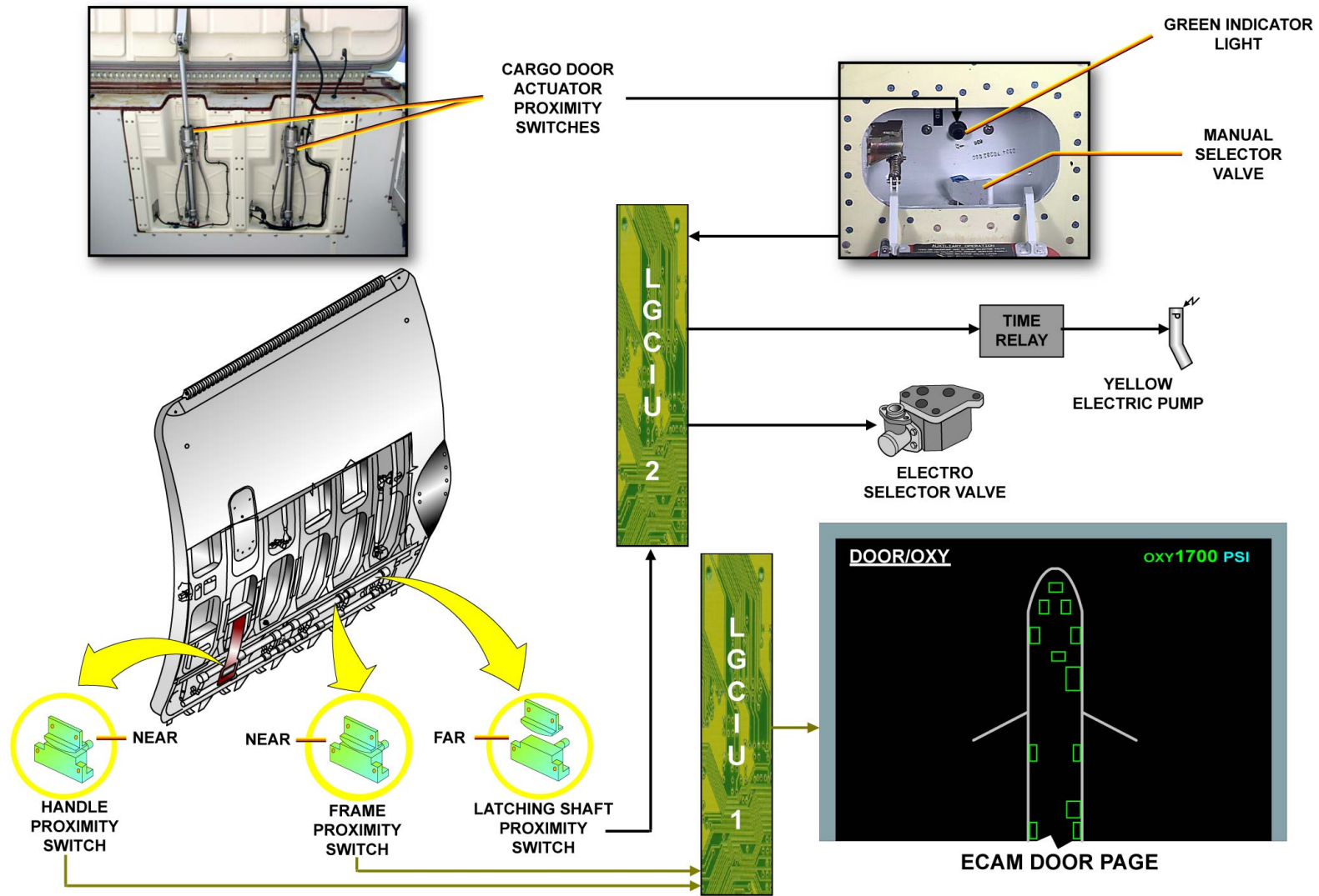
FWD & AFT CARGO DOORS - DOOR INDICATING AND WARNING - PRINCIPLE & DOOR INDICATING AND WARNING - LOCKED
