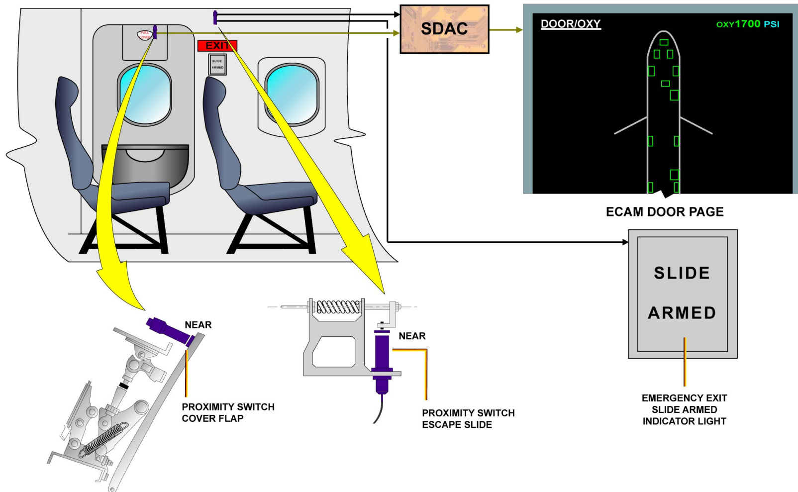
EMERGENCY EXIT DOORS - DOOR INDICATING AND WARNING - PRINCIPLE & DOOR INDICATING AND WARNING - LOCKED
