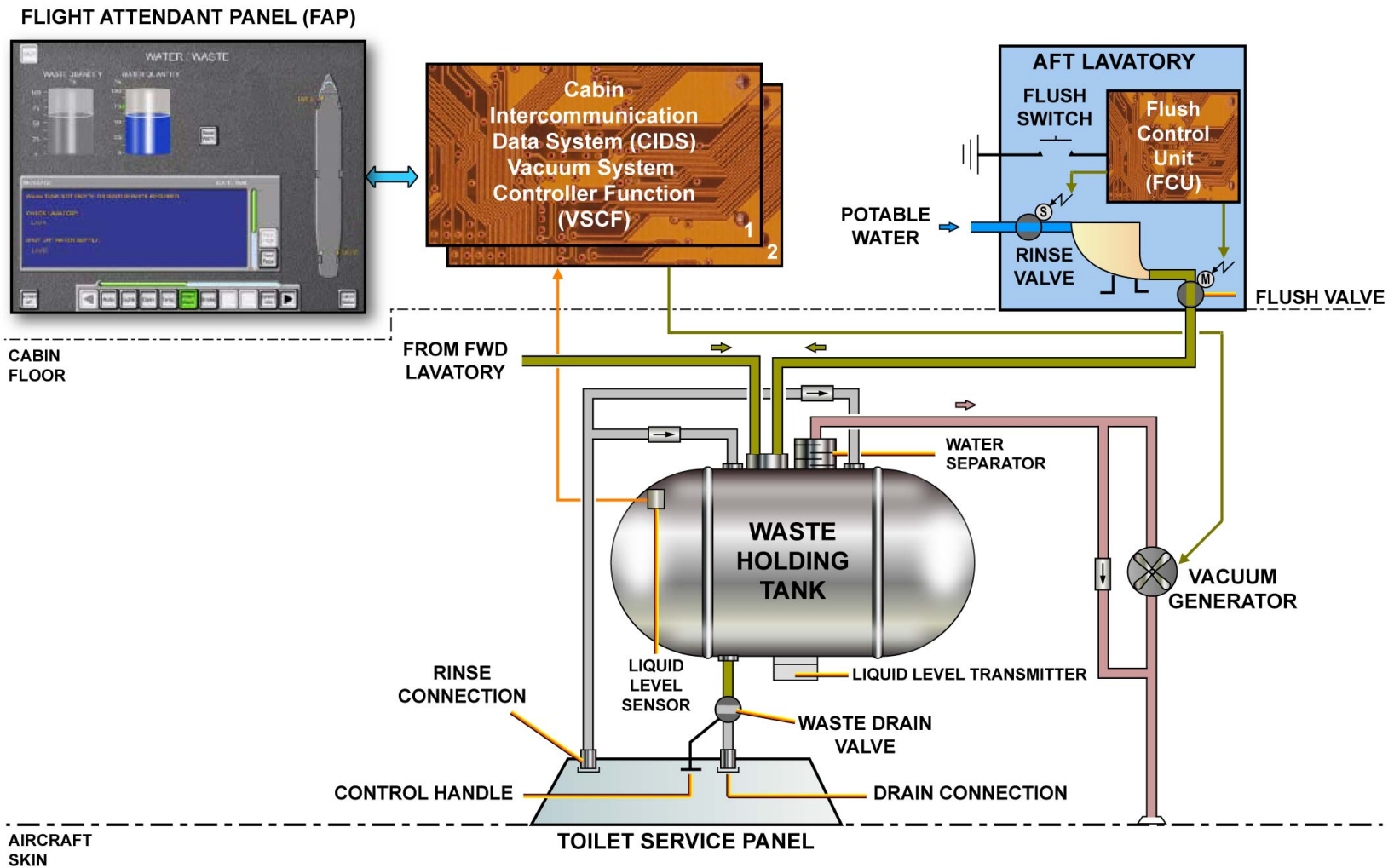
SYSTEM OVERVIEW - TOILET SYSTEM ... TOILET SYSTEM CONTROL AND INDICATING
