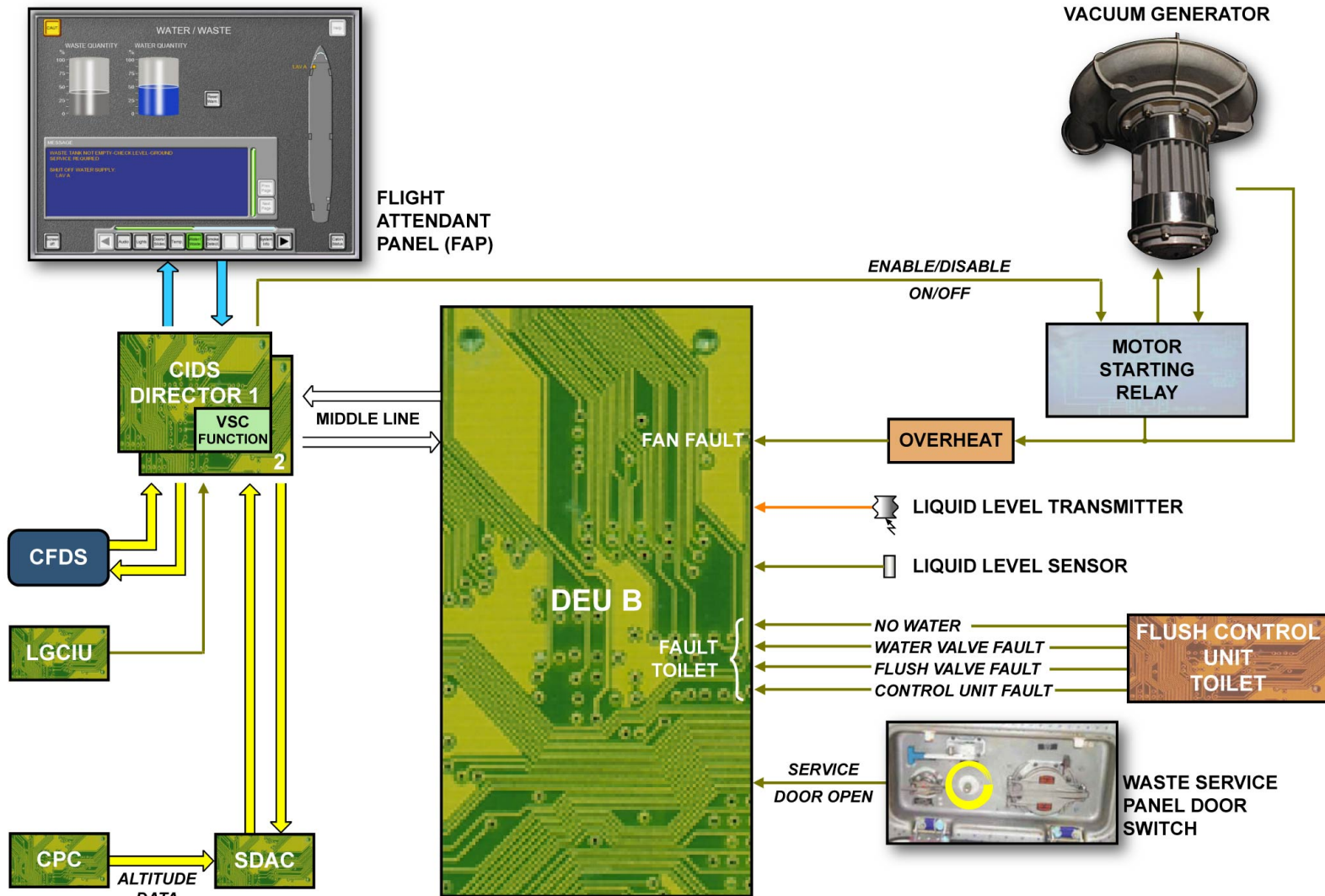
GENERAL ... FAP WATER/WASTE PAGE INDICATING
