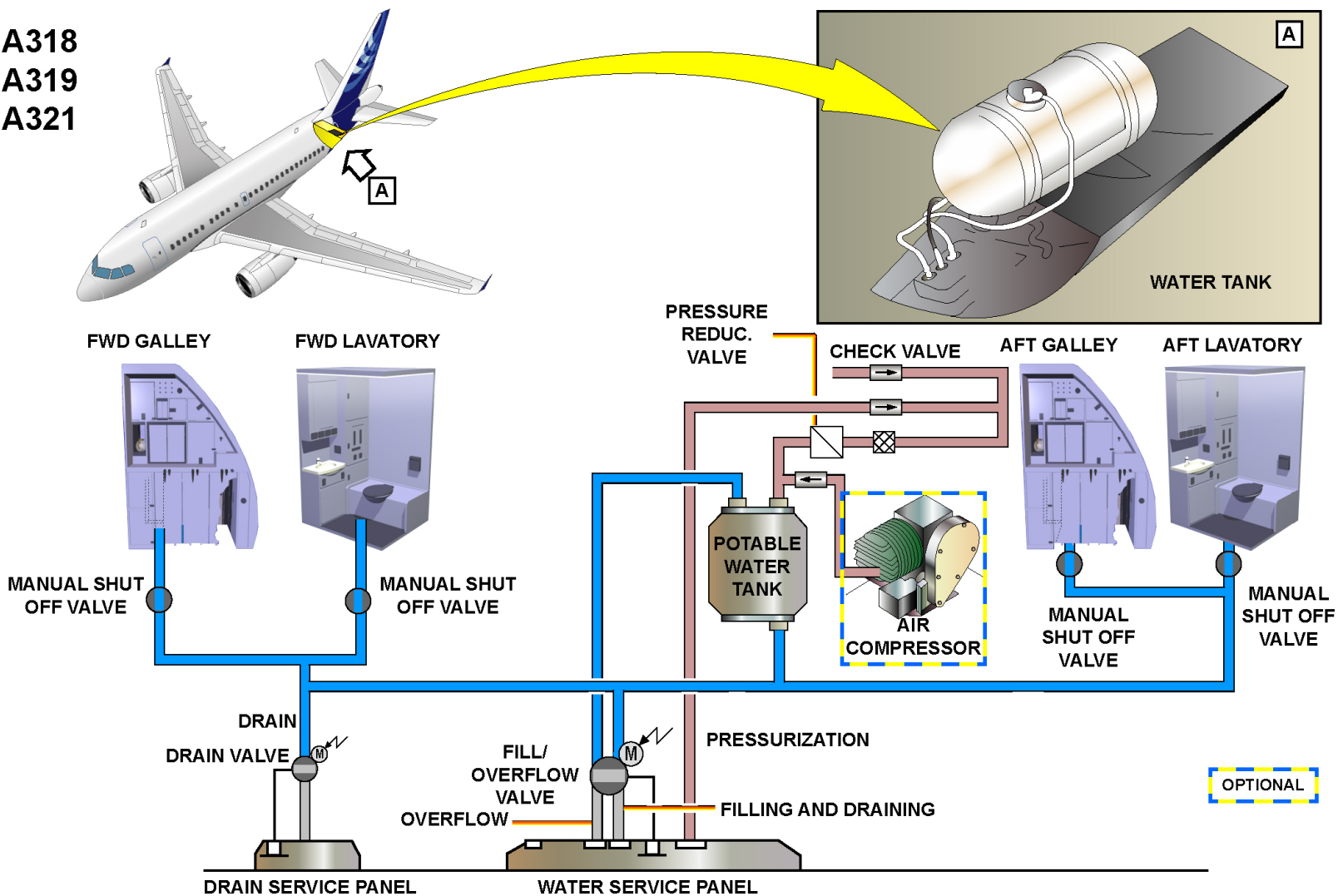
SYSTEM OVERVIEW - WATER FLUID STORAGE (A318 / A319 / A321) & POTABLE WATER SYSTEM
