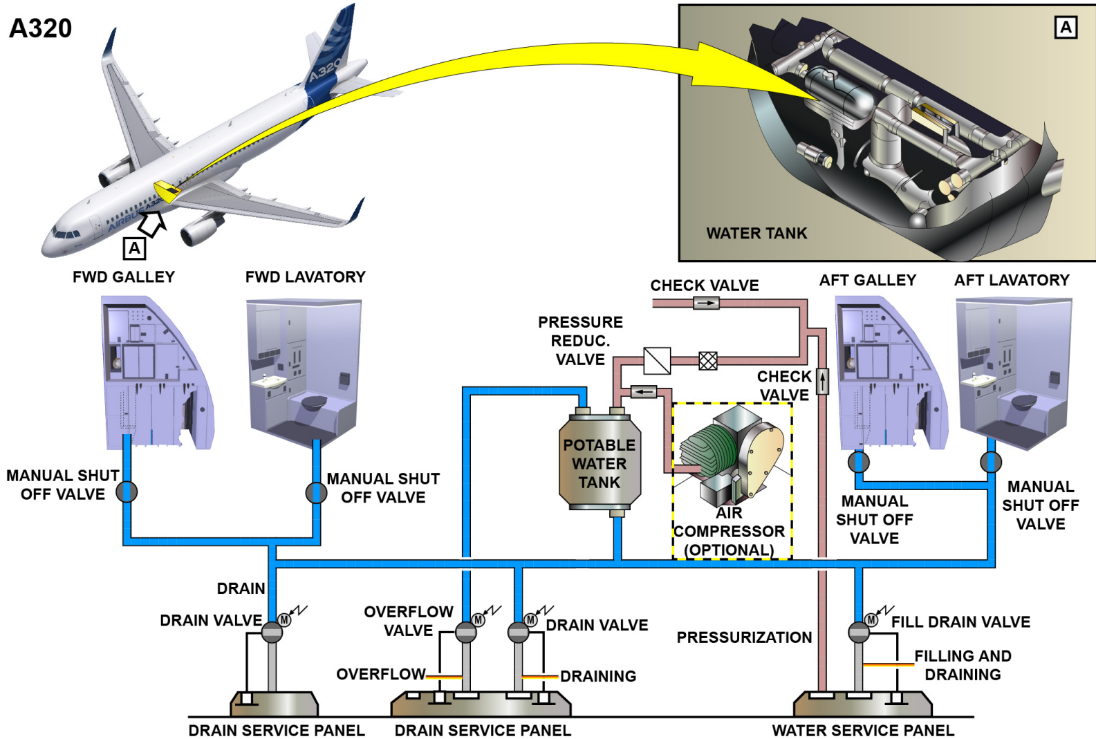
SYSTEM INTRODUCTION & POTABLE WATER SYSTEM
