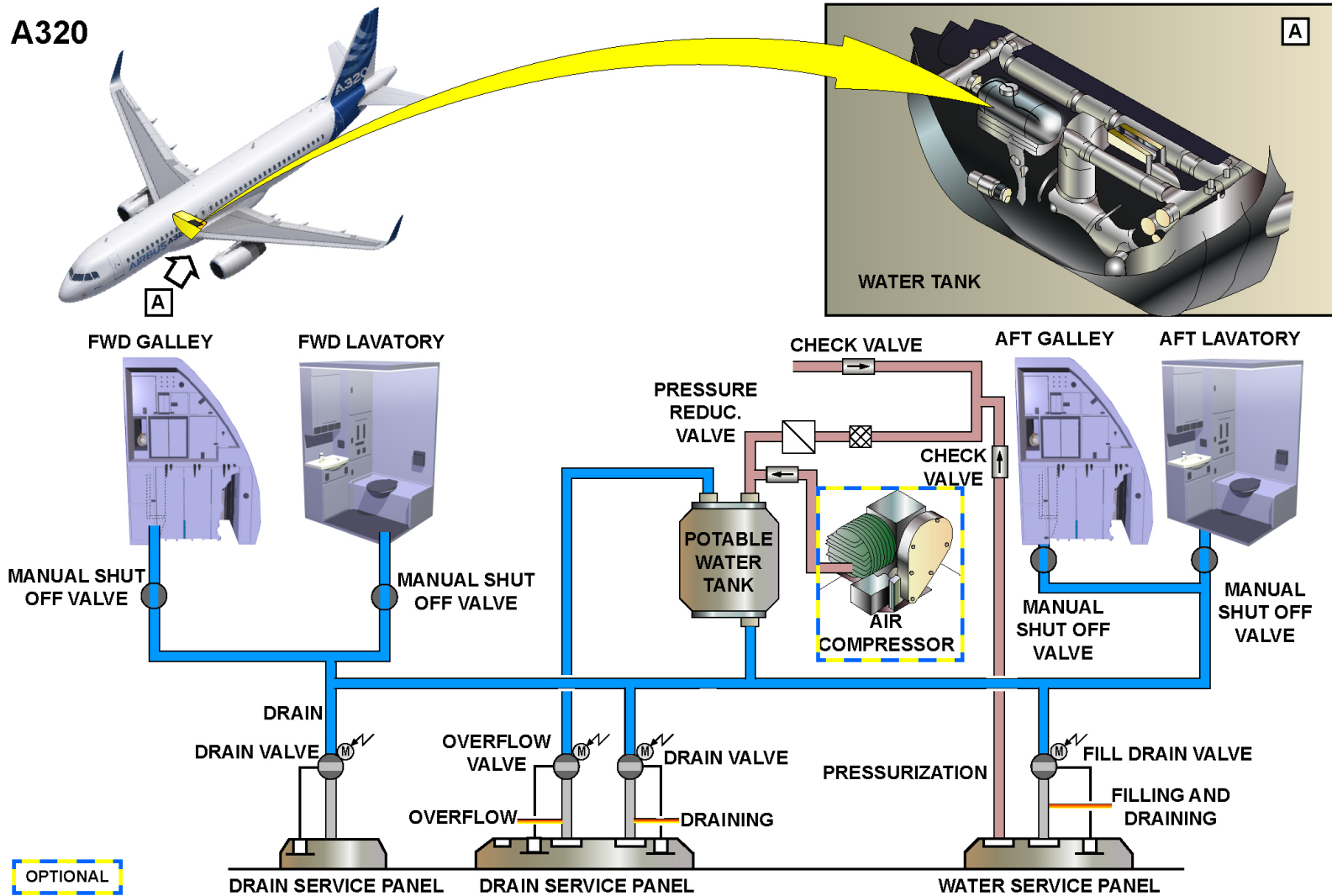
SYSTEM OVERVIEW - WATER FLUID STORAGE (A320)
