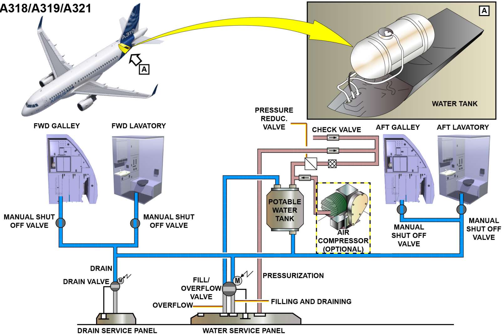
POTABLE WATER SYSTEM - A318/A319/A321
