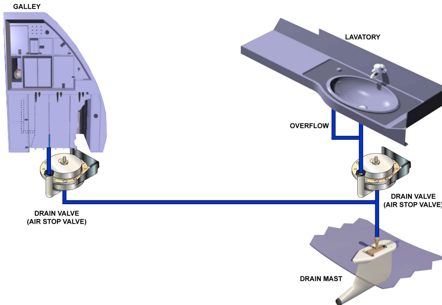
WASTE WATER SYSTEM
