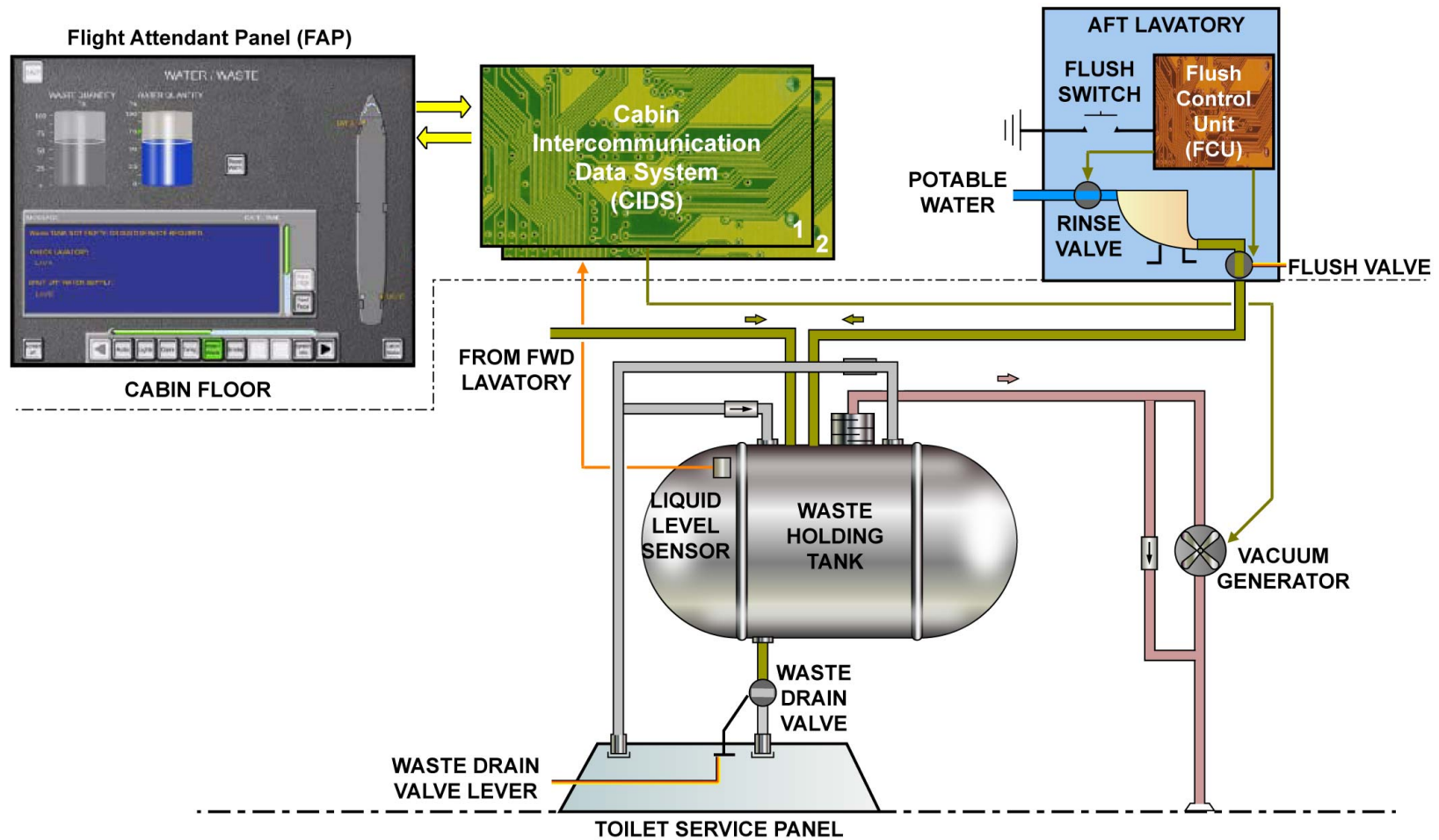
VACUUM TOILET SYSTEM - FLUSHING
