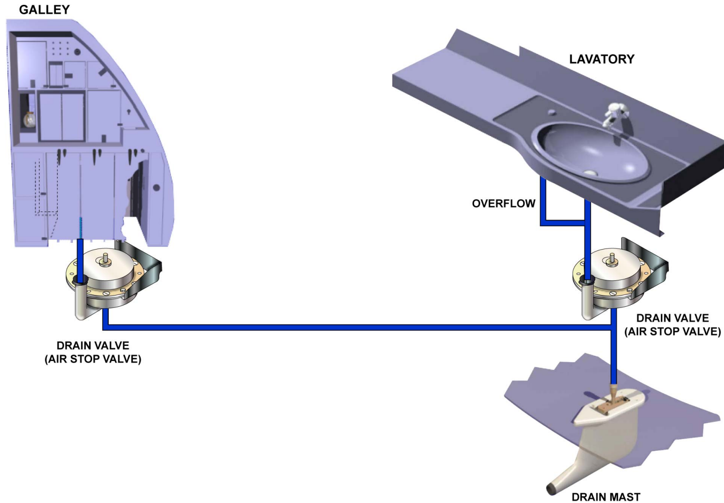
SYSTEM OVERVIEW - WASTE WATER SYSTEM
