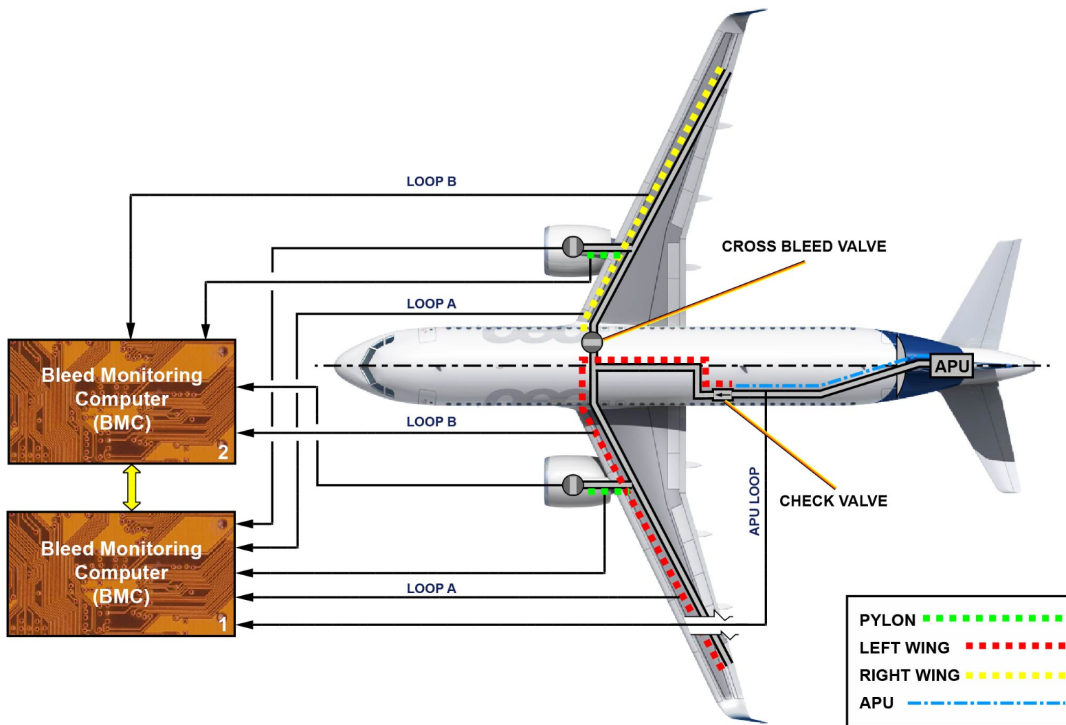
SYSTEM OVERVIEW - LEAK DETECTION
