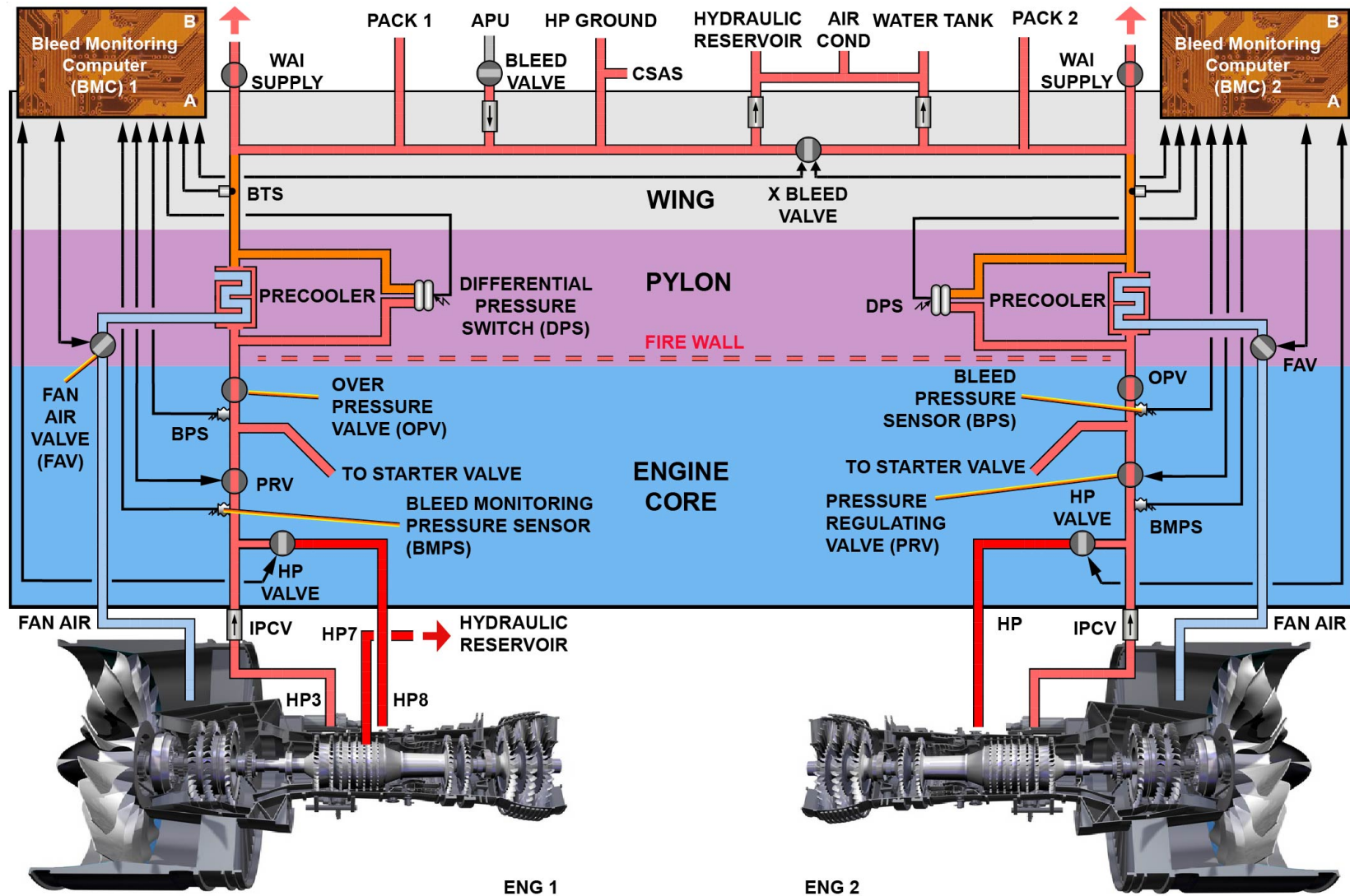
SYSTEM OVERVIEW - ENGINE BLEED &amp; APU BLEED/EXTERNAL AIR
