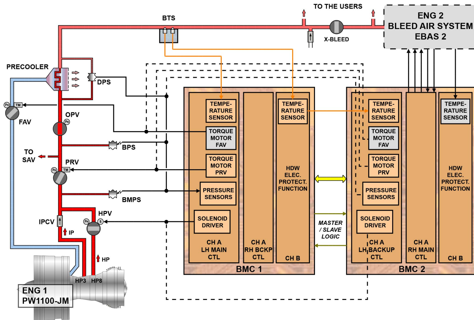
BLEED TEMPERATURE SENSOR (BTS)
