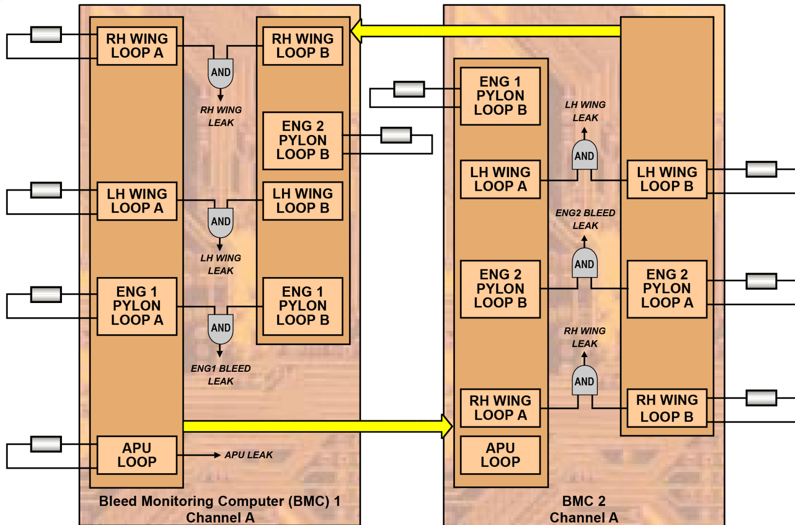
DETECTION LOGIC
