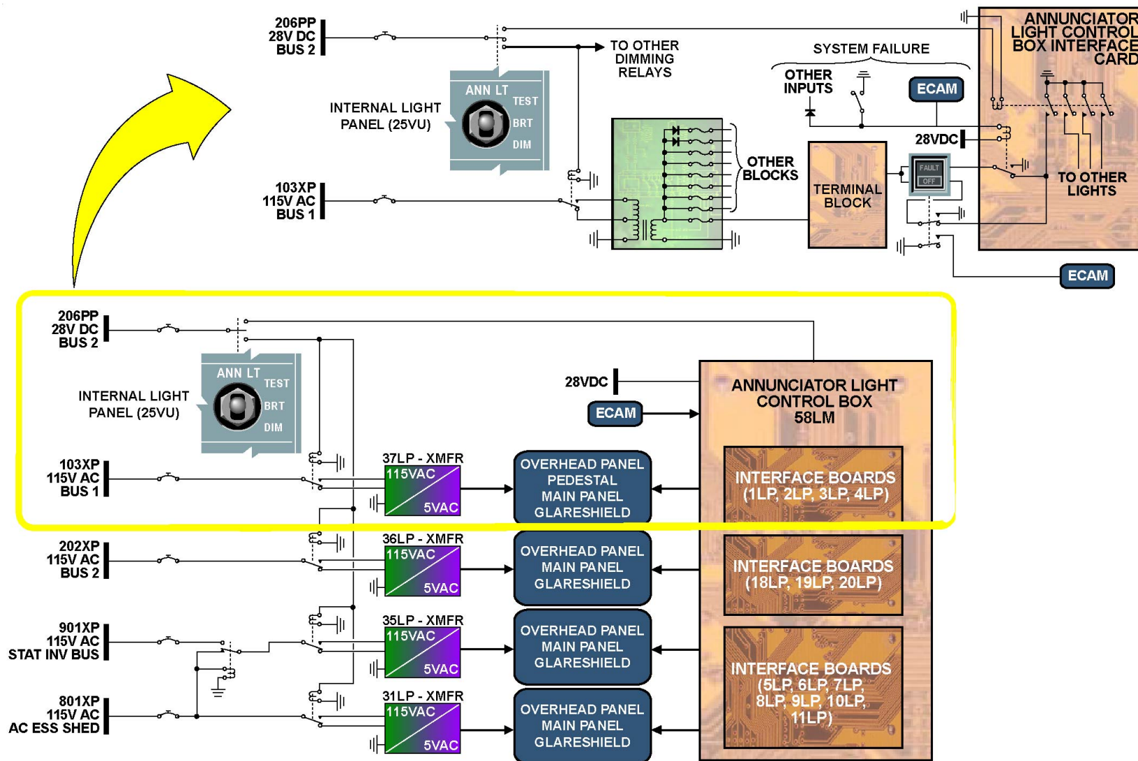
SYSTEM DESCRIPTION - TRANSFORMERS ... FOUR-STAGES RELAY
