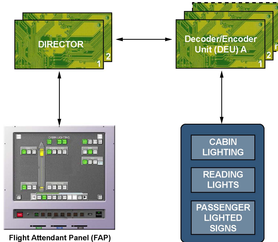
CABIN LIGHTS - CABIN LIGHTS THROUGH CIDS
